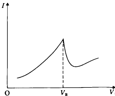
1.19 The current variation with voltage in a Franck-Hertz experiment.
